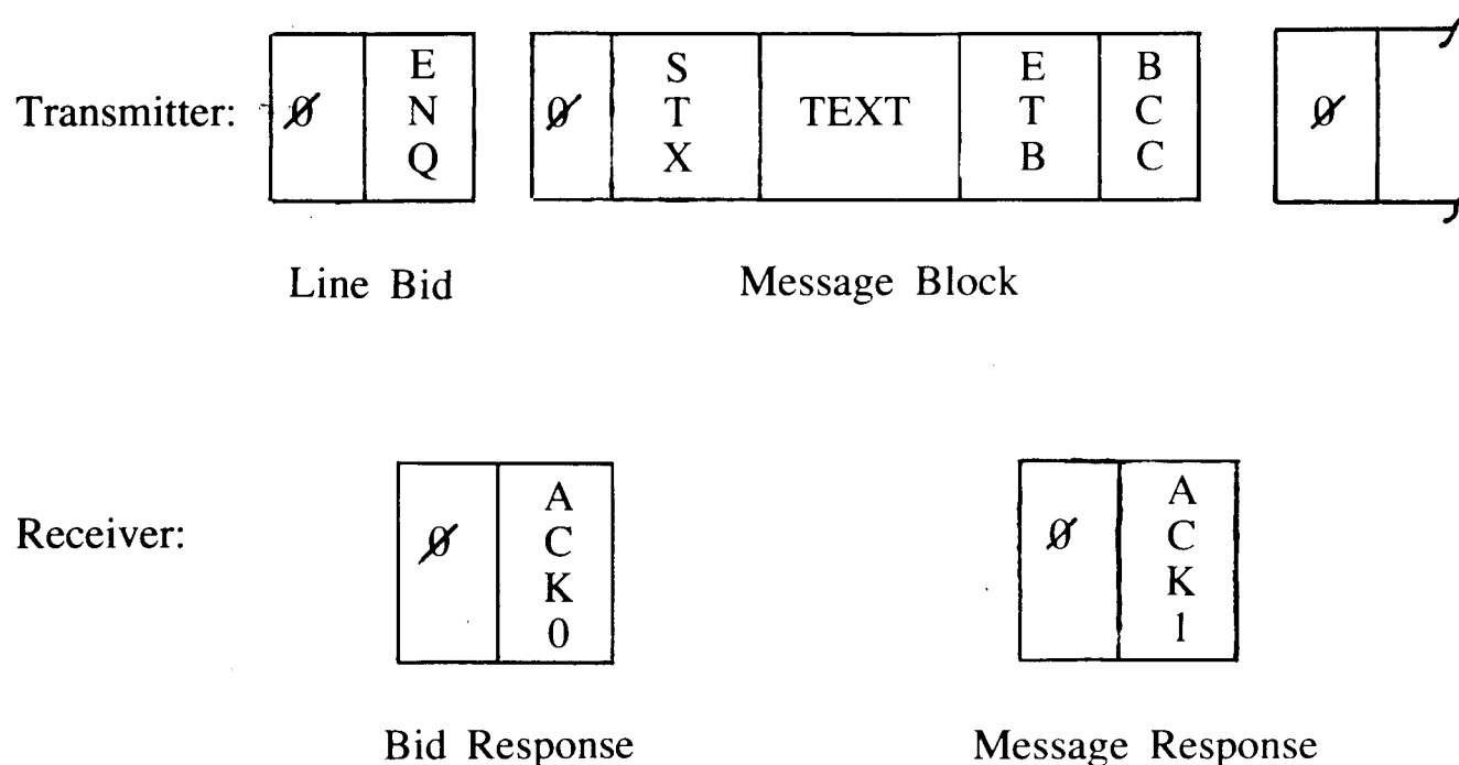
Figure 4. Line Bid Processing (Point-to-Point Operation)
